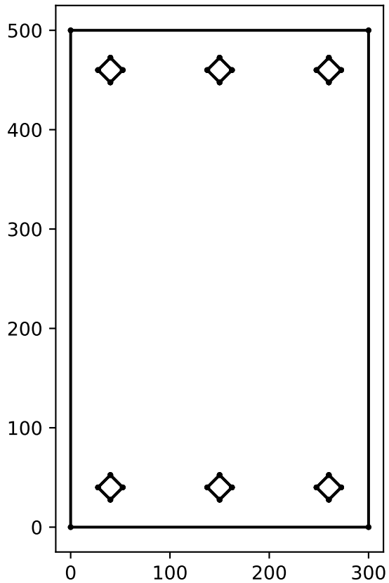
Cross-Section Geometry
