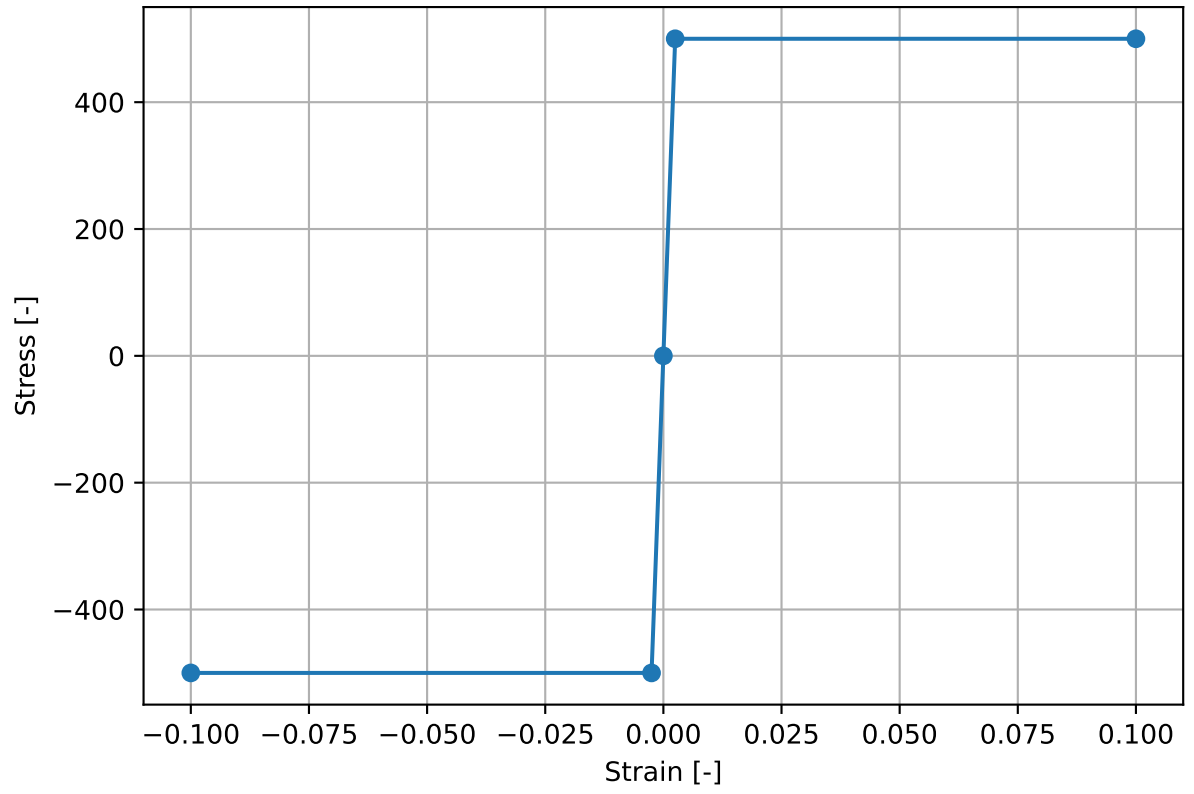
500 MPa Steel (NZS3101:2006) - Stress-Strain Profile
