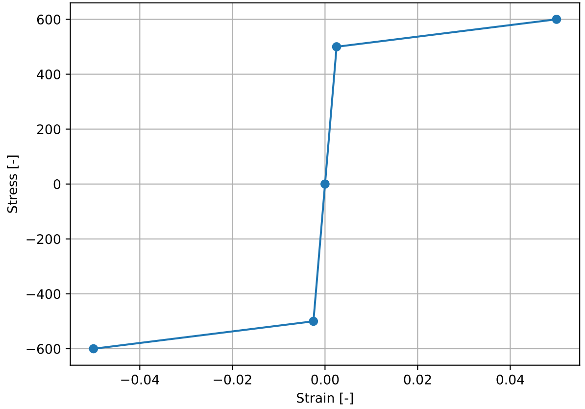
Stress-Strain Profile
