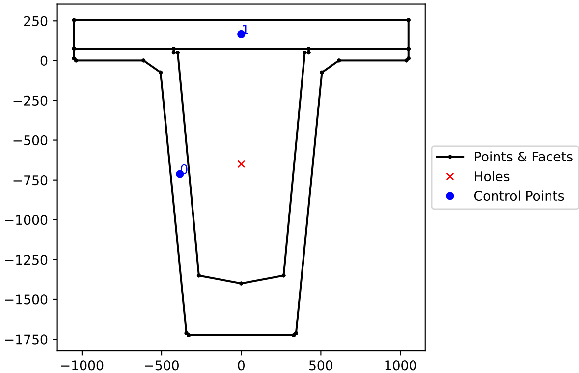
Cross-Section Geometry
