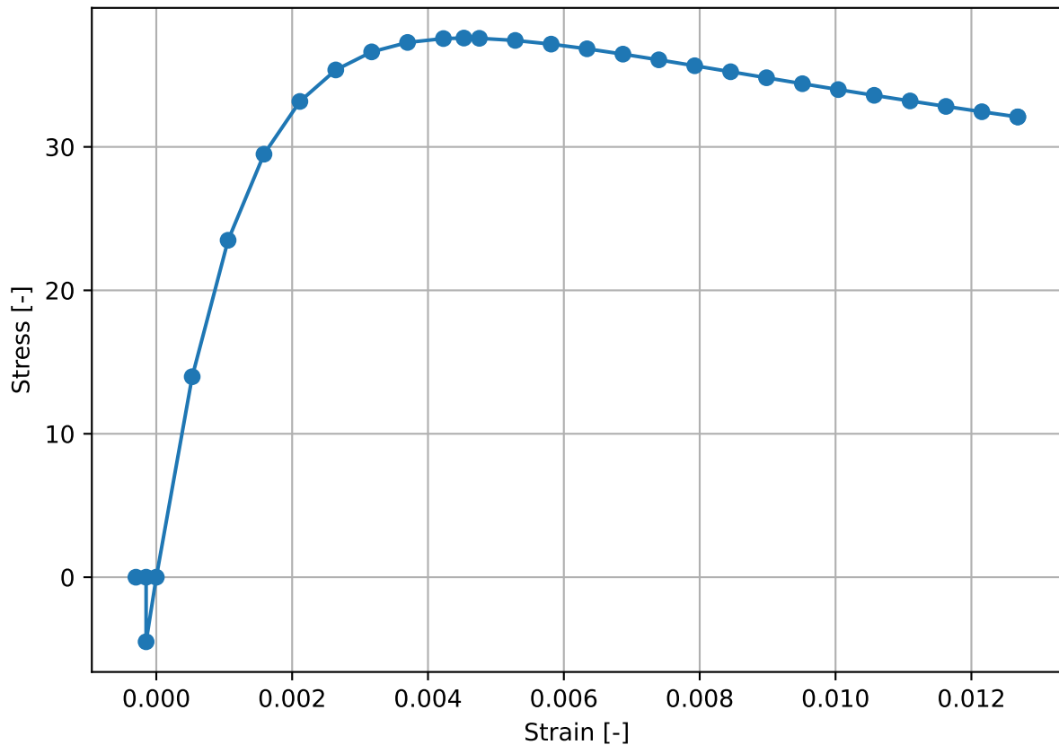
Stress-Strain Profile
