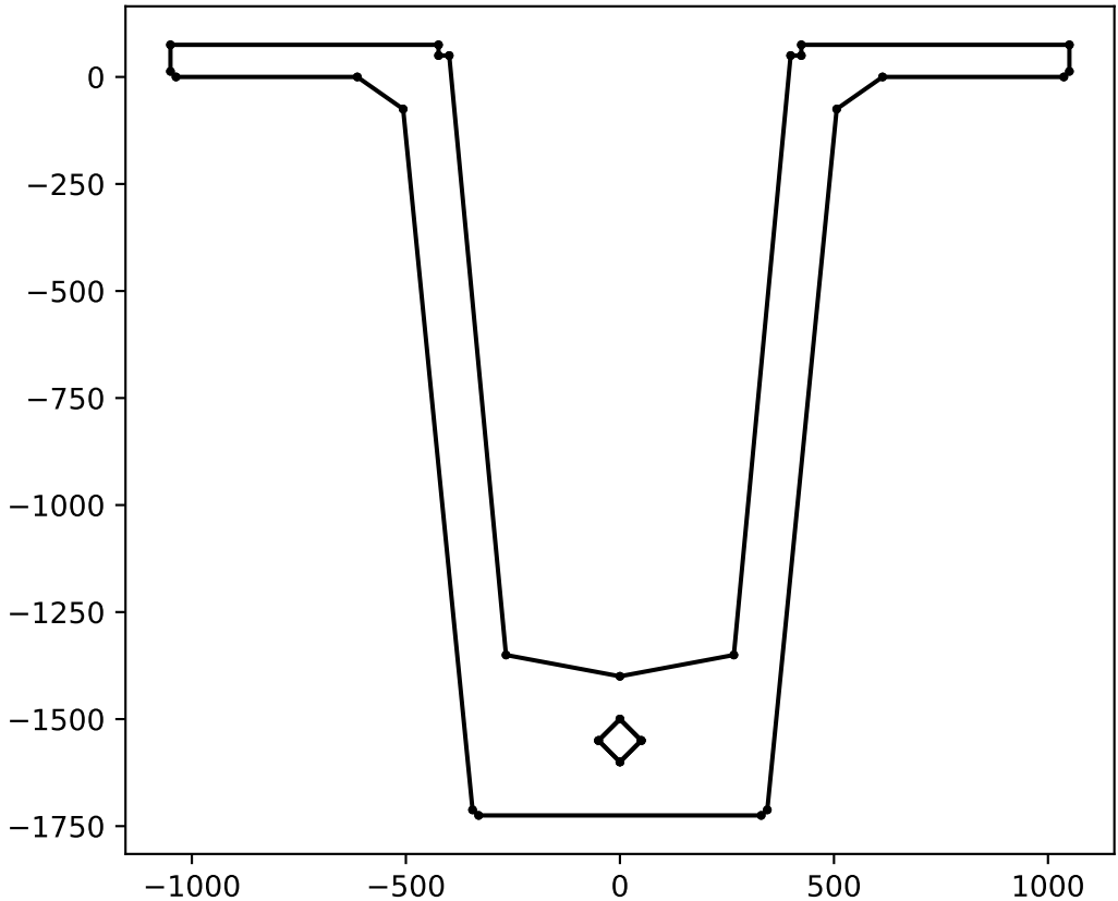
Cross-Section Geometry
