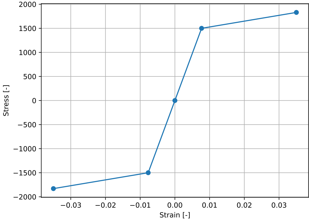
Stress-Strain Profile
