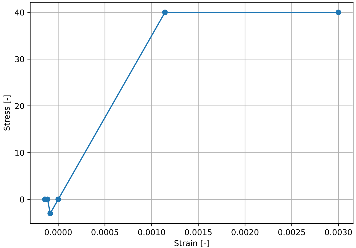
Stress-Strain Profile
