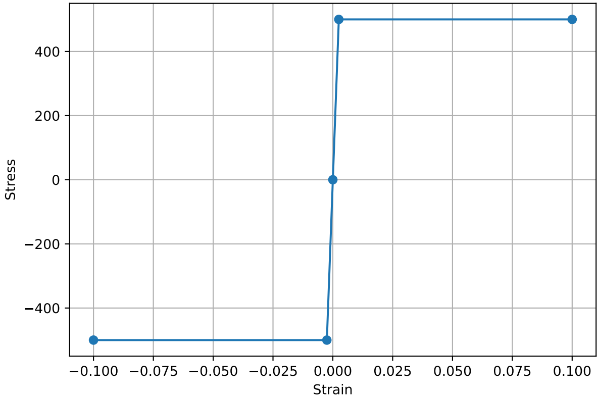
500 MPa Steel (NZS3101:2006) - Stress-Strain Profile
