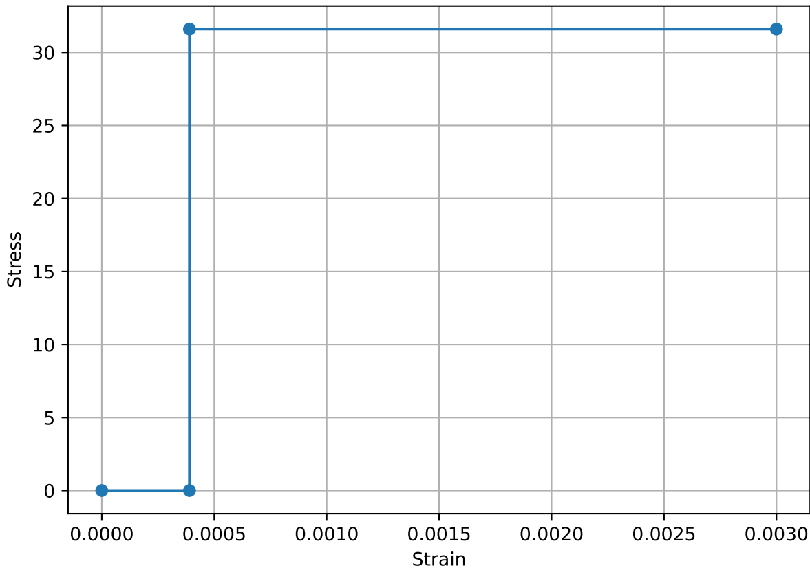
40 MPa Concrete (AS 3600:2018) - Ultimate Profile
