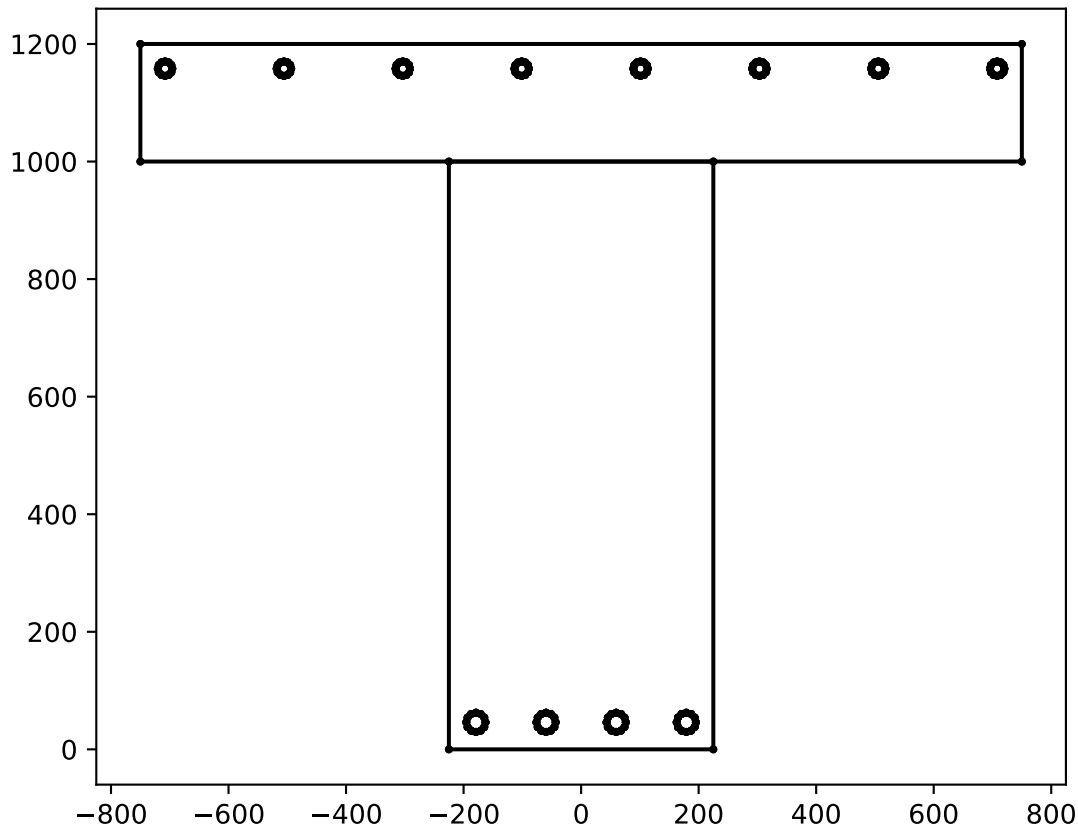
Cross-Section Geometry
