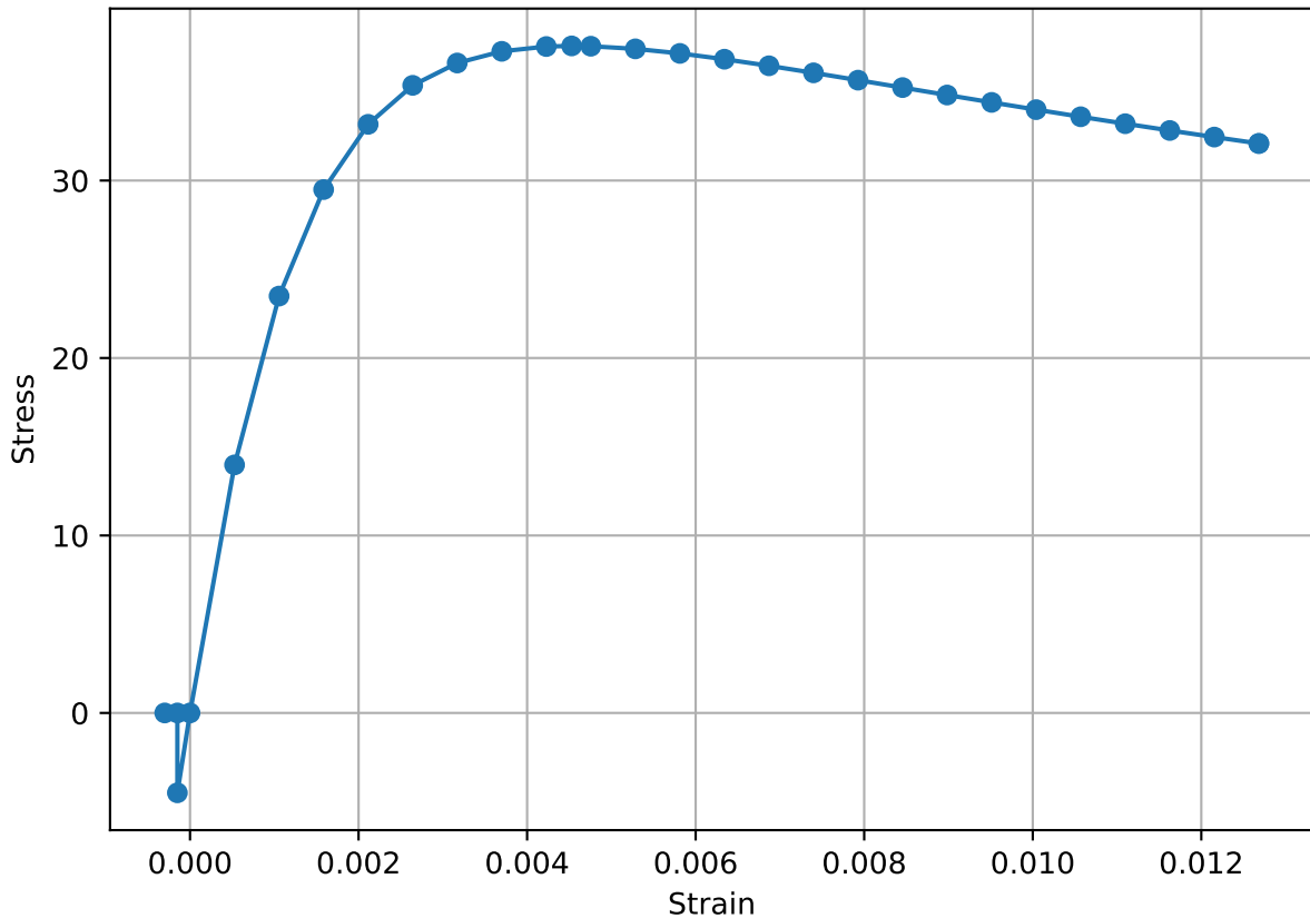
Stress-Strain Profile
