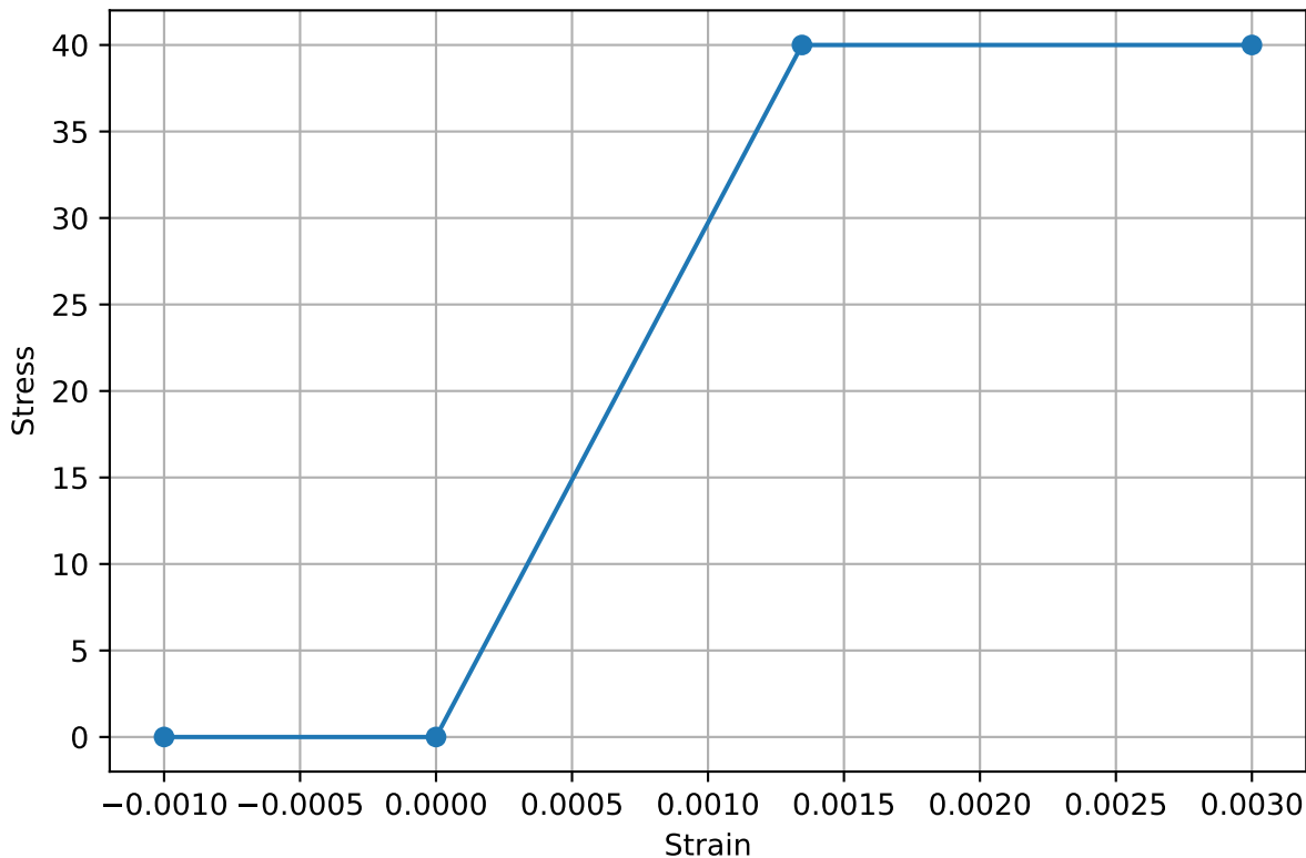
40 MPa Conc [2300 kg/m 3 ] (NZS3101:2006) - Service Profile
