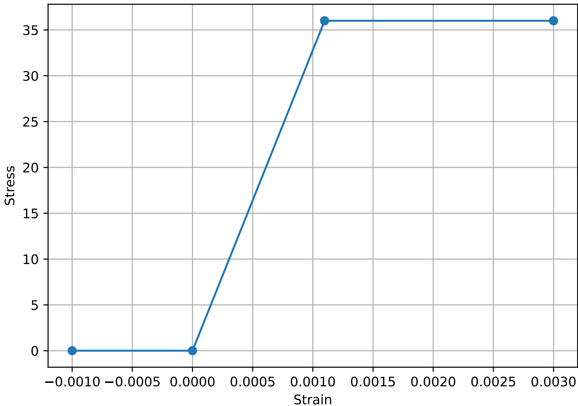
40 MPa Concrete (AS 3600:2018) - Service Profile
