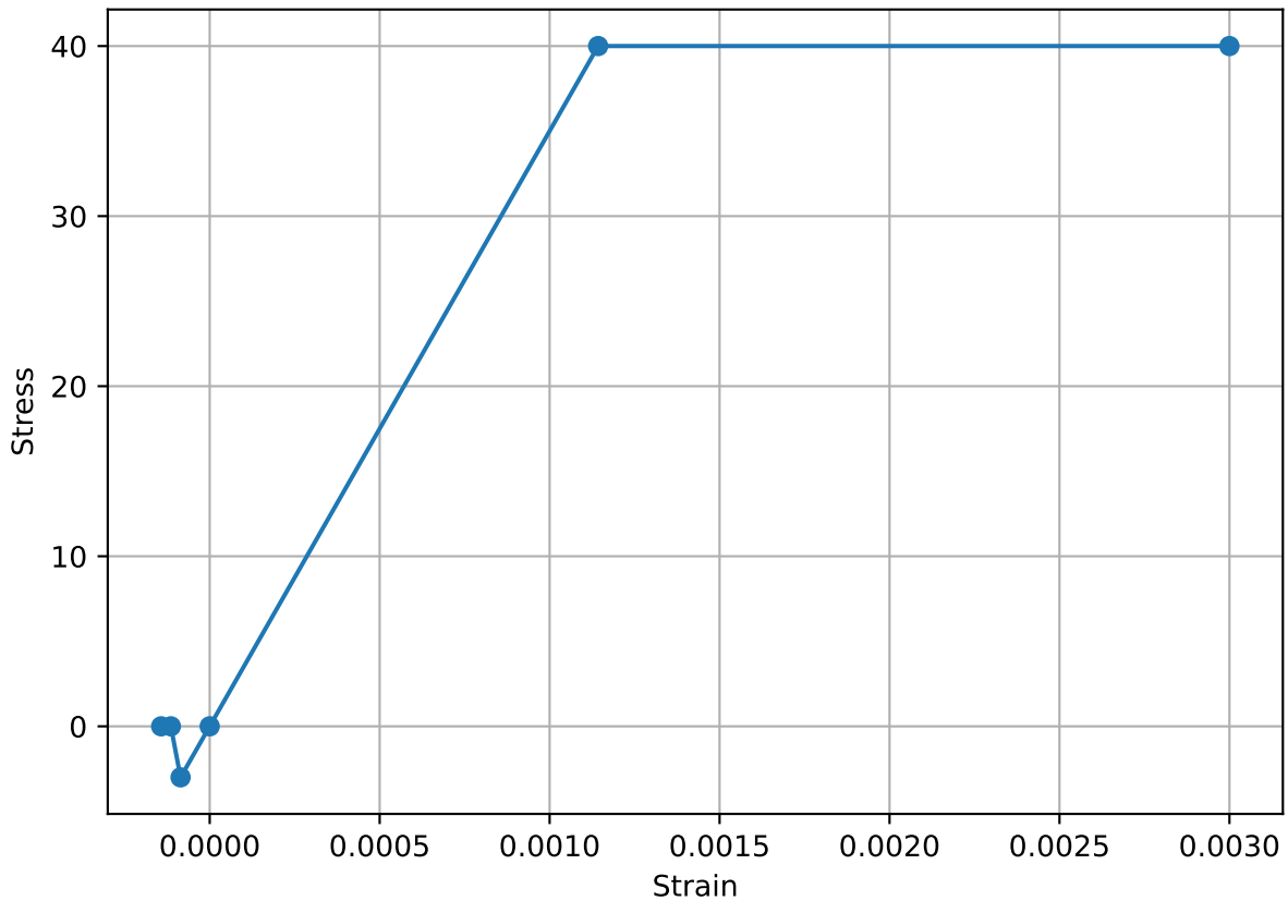
Stress-Strain Profile
