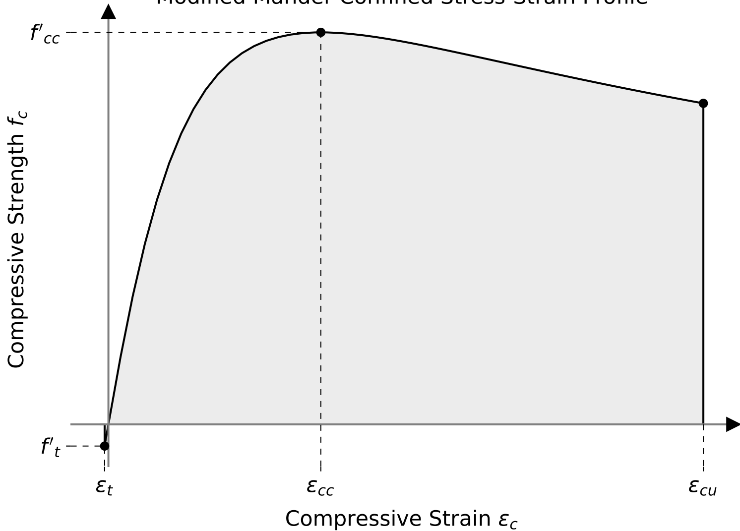
Modified Mander Confined Stress-Strain Profile
