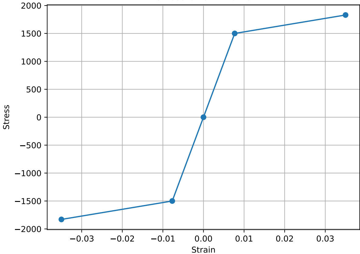
Stress-Strain Profile
