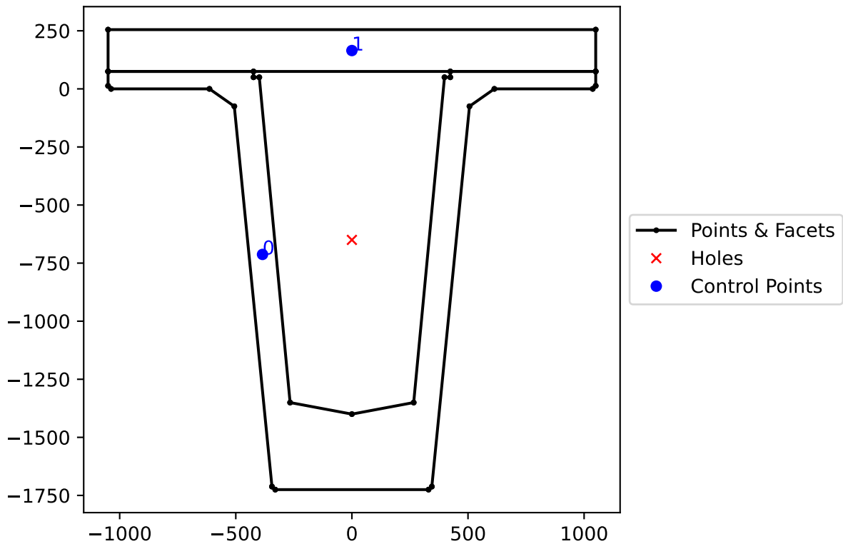
Cross-Section Geometry
