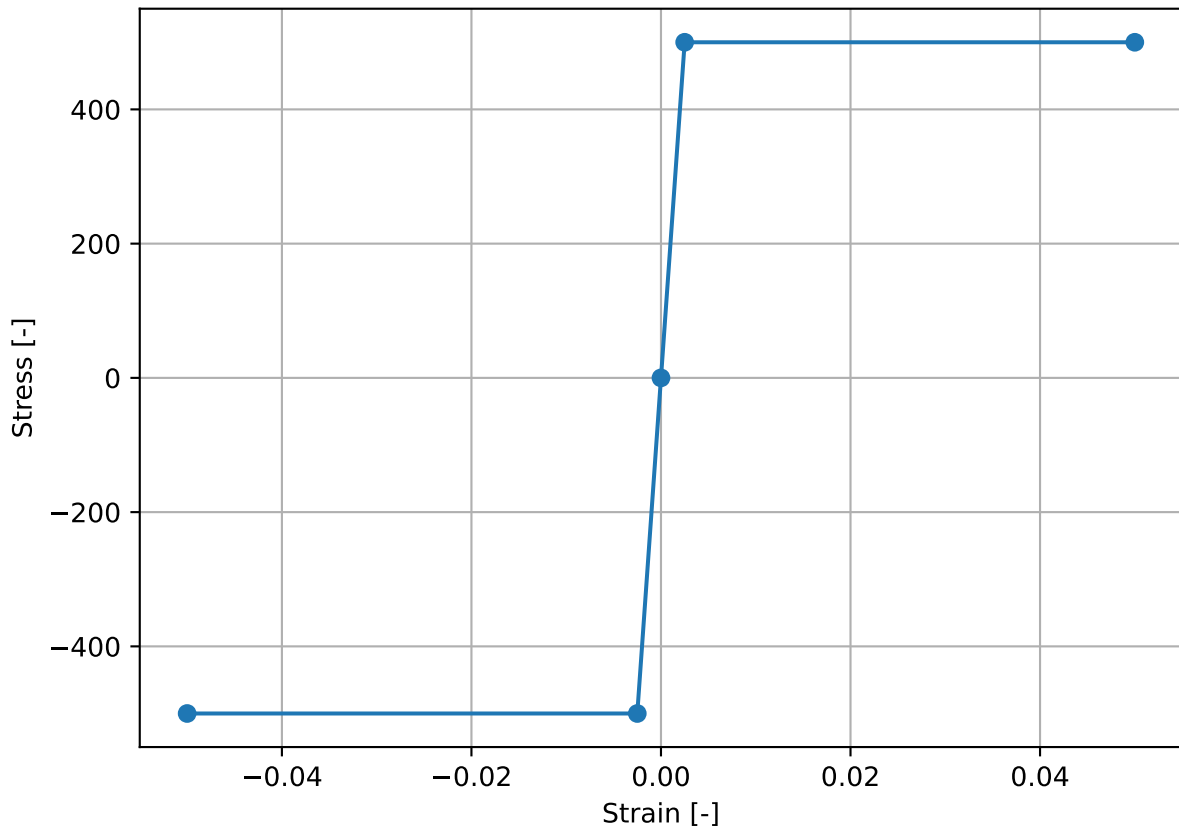
500 MPa Steel (AS 3600:2018) - Stress-Strain Profile
