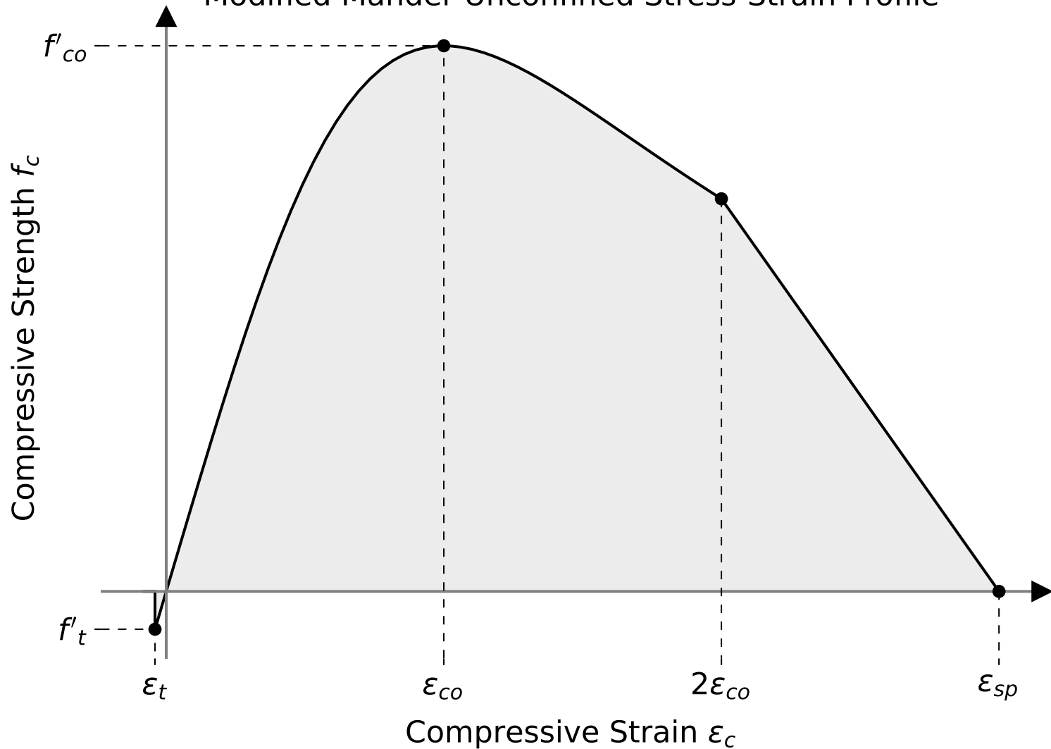
Modified Mander Unconfined Stress-Strain Profile
